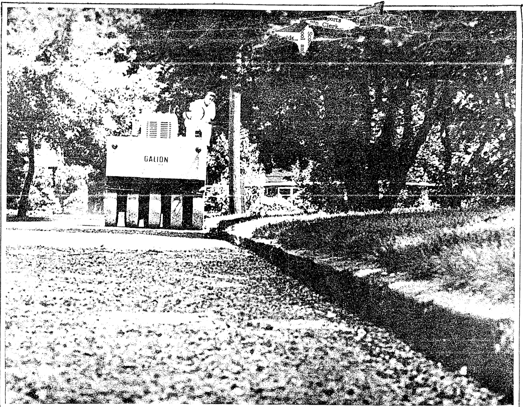
ROLLING ALONG ---This is a new piece of equipment used by the Scotch Plains Department of Public Properties to assist in their street preaving project. Instead of the conventional flat steel rollers, the new machine has overlapping rubber tires that can more effectively reach uneven planes. The workings of the department under the direction of Alex Milton is the subject of a feature story in this week's issue. (Staff Photo)
